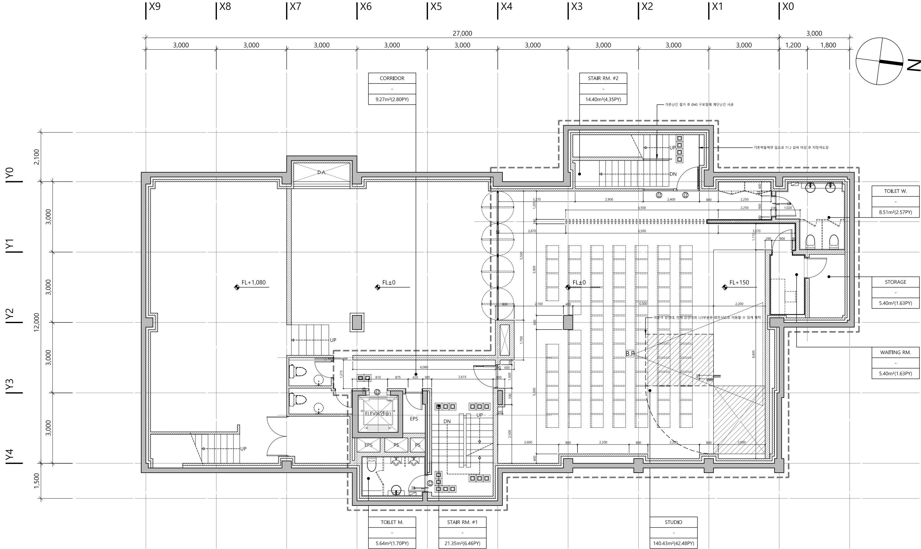
1 B1F FLOOR PLAN A-100 SCALE : 1 / 100
